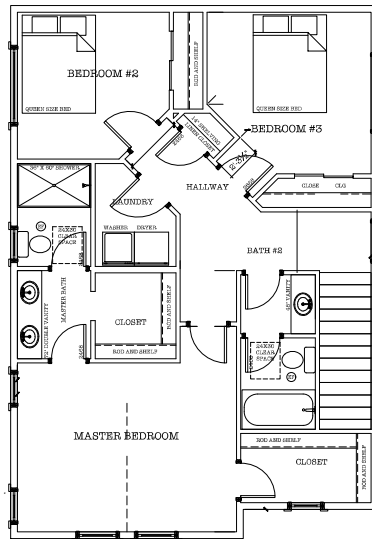
UPPER LEVEL FLOOR PLAN SCALE: 1/4" = 1'-0"
